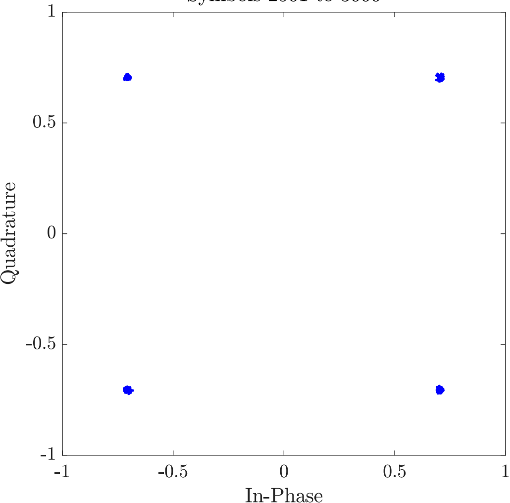
Adaptive filter (CMA) with 19 taps Symbols 2501 to 3000
