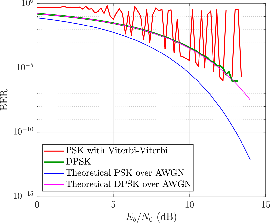
QPSK with phase noise and correction 10^6 bits, LO 5 MHz, blocksize 40 Sa
