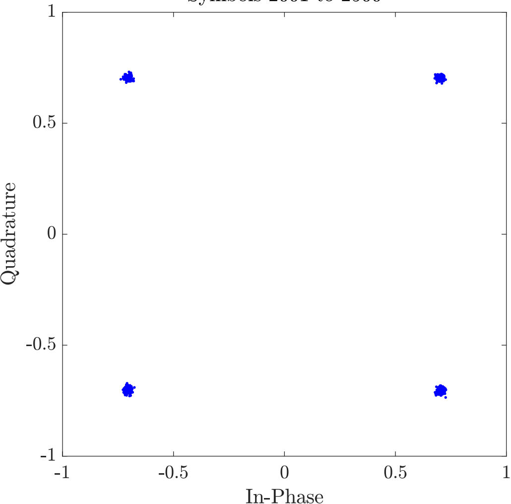
Adaptive filter (CMA) with 19 taps Symbols 2001 to 2500
