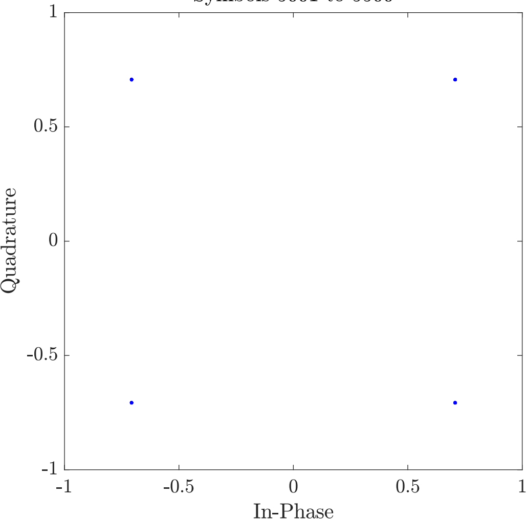
Adaptive filter (CMA) with 19 taps Symbols 5001 to 5500
