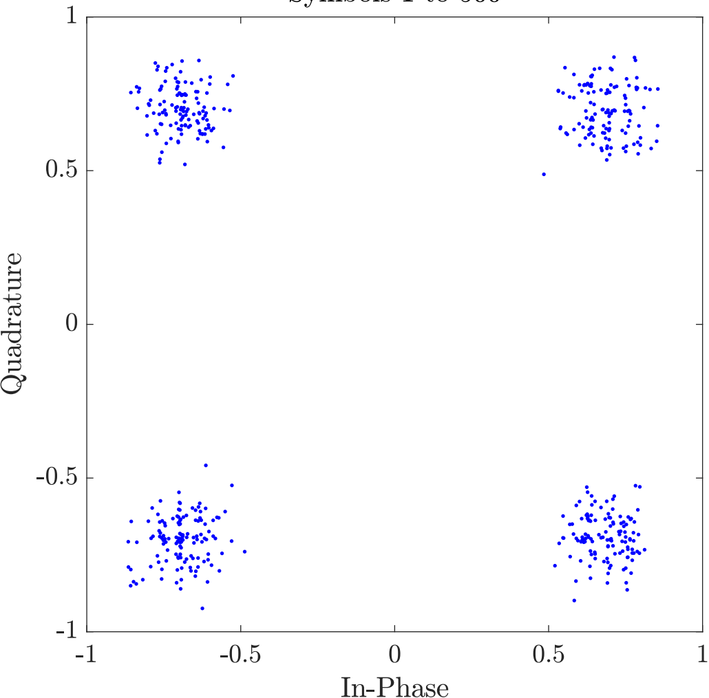
Adaptive filter (CMA) with 19 taps Symbols 1 to 500
