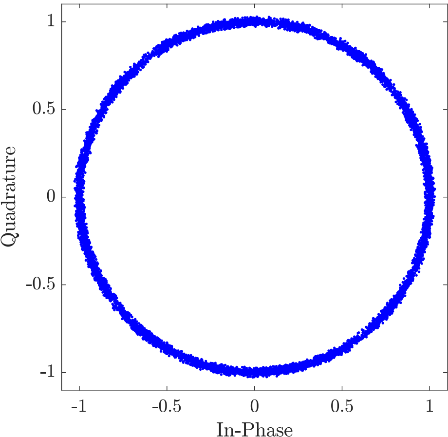
QPSK constellation with phase noise
