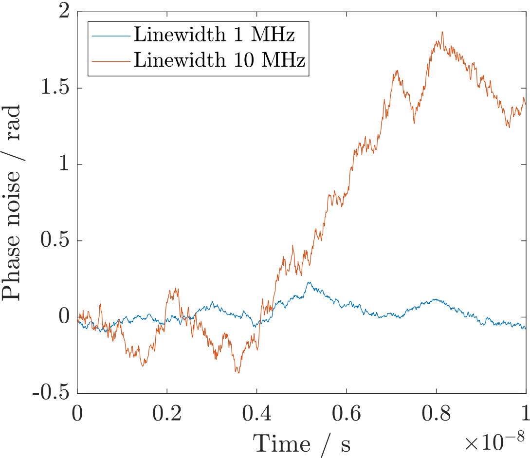
Phase noise of lasers with different linewidths
