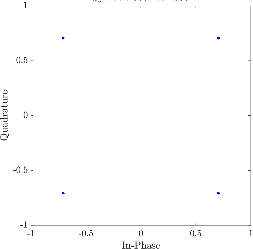
Adaptive filter (CMA) with 19 taps Symbols 3501 to 4000
