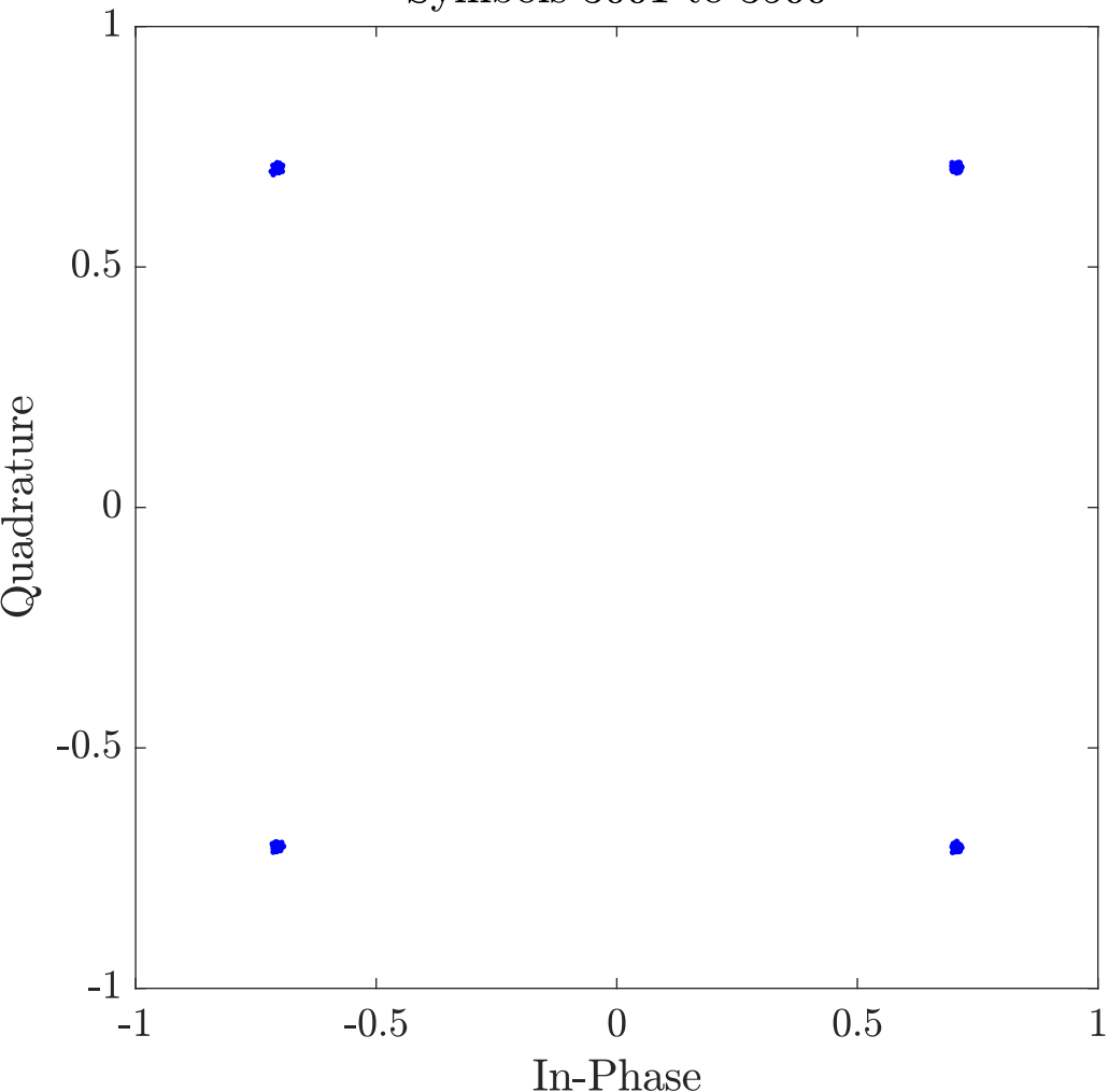
Adaptive filter (CMA) with 19 taps Symbols 3001 to 3500
