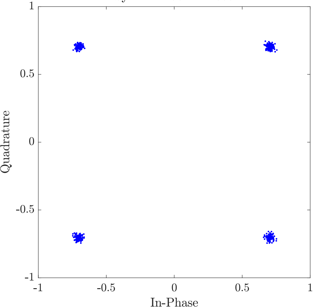
Adaptive filter (CMA) with 19 taps Symbols 1501 to 2000
