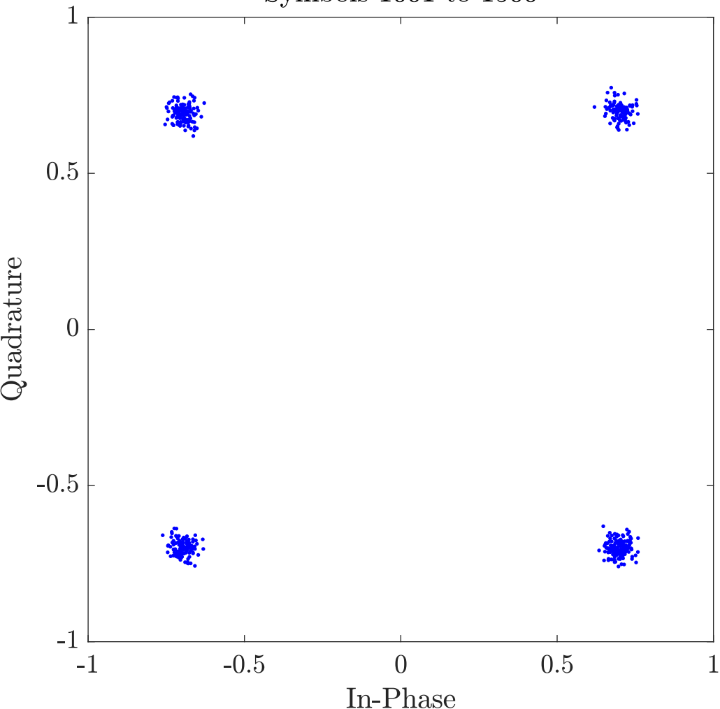
Adaptive filter (CMA) with 19 taps Symbols 1001 to 1500
