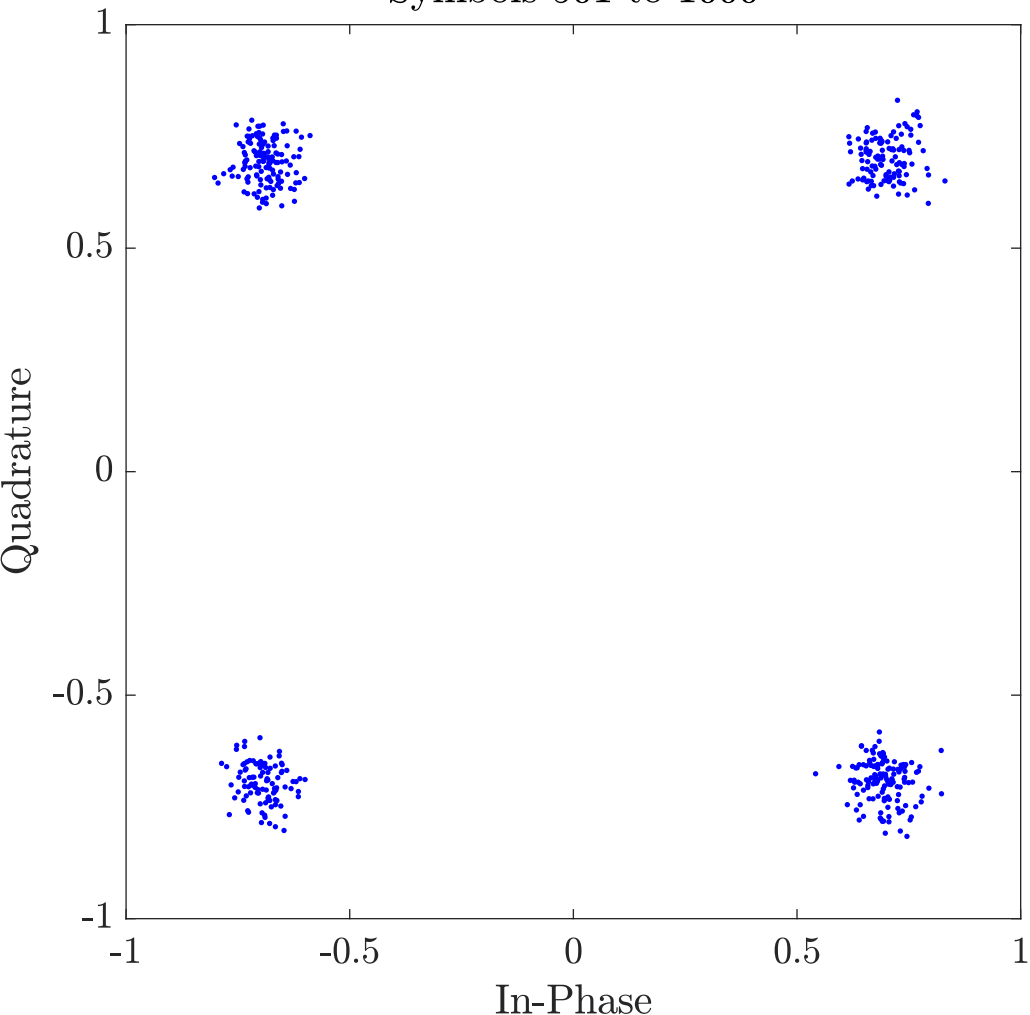
Adaptive filter (CMA) with 19 taps Symbols 501 to 1000
